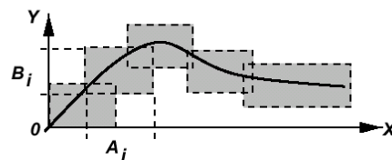
Figure 8. Fuzzy graph of a function.
