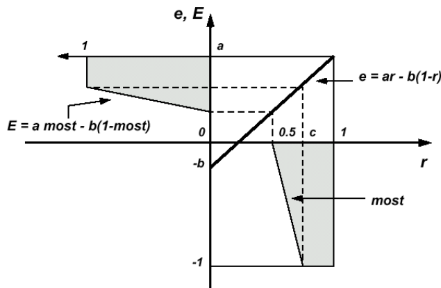
Figure 21. Computation of expectation through use of the extension principle.
