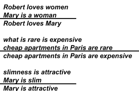
Figure 5 (b) Examples of incorrect reasoning.
