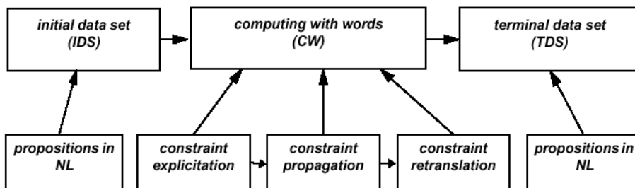
Figure 13. Conceptual structure of computing with words.
