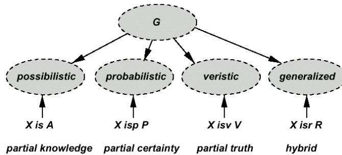
Figure 3 (b) Principal types of granules.
