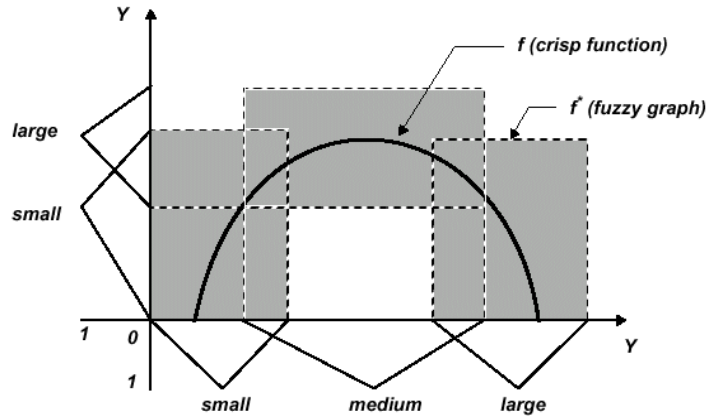
Figure 8. Fuzzy graph of a function.
