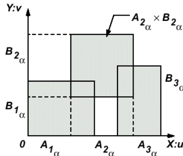
Figure 16. \alpha -Cuts of a function described by a fuzzy graph.
