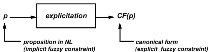
Figure 12. Canonical form of a proposition.
