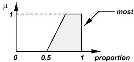
Figure 20. Membership function of most .
