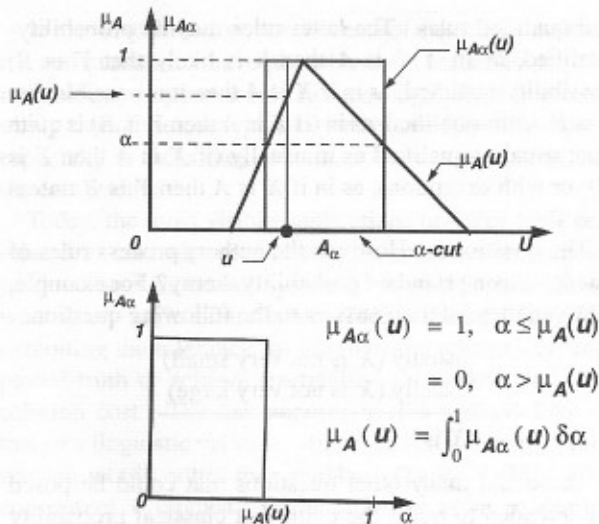
Figure 2. Additive Decomposition of a Fuzzy Set. The \alpha cuts form a continuum.
