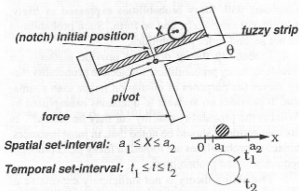
Figure 4. The Fuzzy Ball-and-Beam Problem. The ball rolls/slides on a fuzzy strip, which is attached to a beam.
